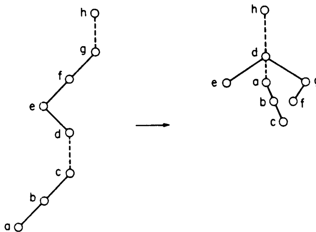
FIG. 17. Splaying at a node a in a lexicographic splay tree. Subtrees of nodes along the access path are deleted for clarity.
