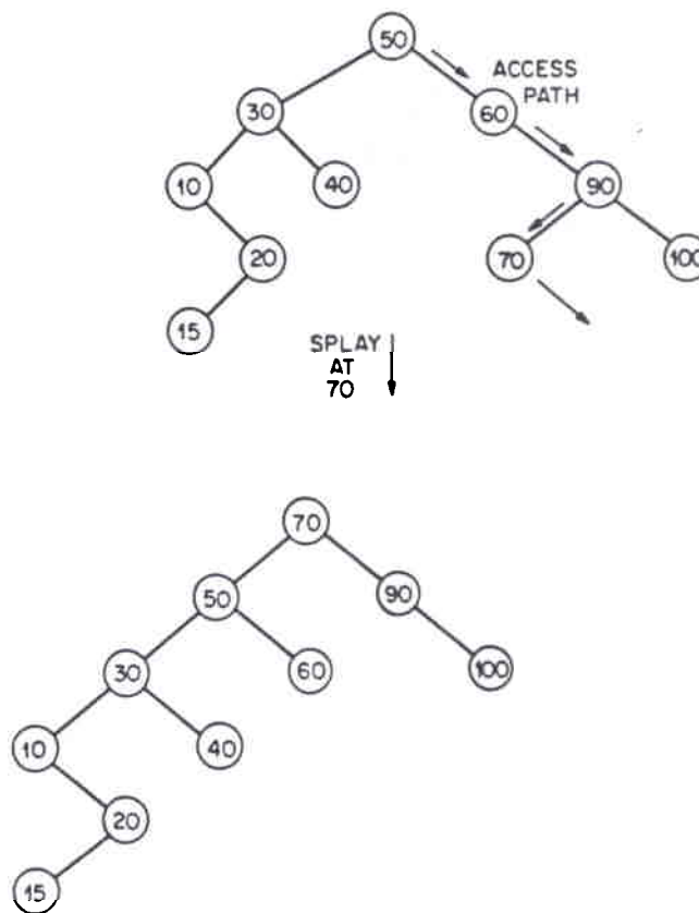
FIG. 6. Splaying after an unsuccessful access of item 80.
