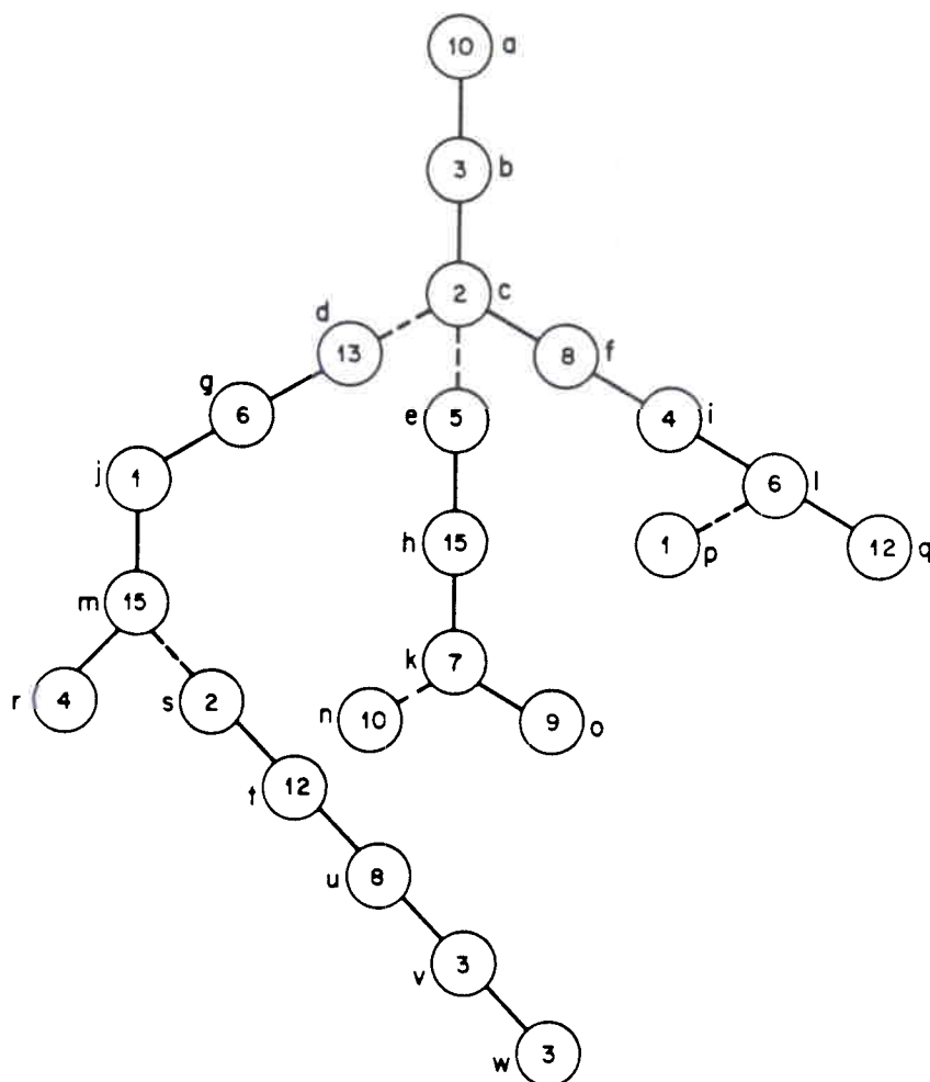
FIG. 19a. Virtual tree representing a link/cut tree: Actual tree. Numbers in nodes are costs. Dashed edges separate parts corresponding to solid subtrees in virtual tree.
